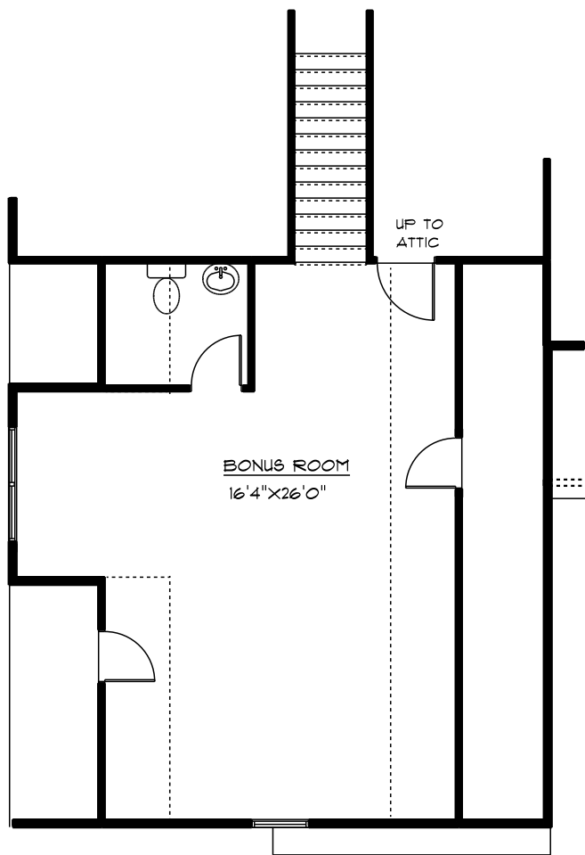
BONUS ROOM PLAN RETREAT MODEL
