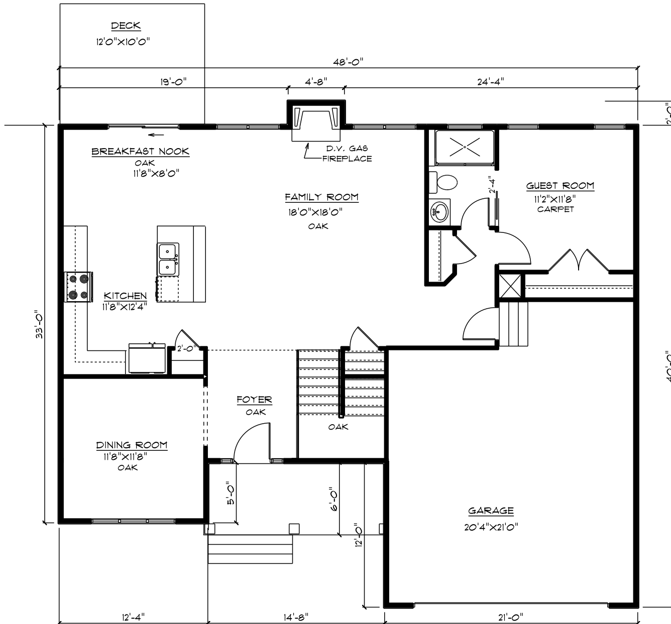
FIRST FLOOR PLAN LOT 15, FENTON MILL ELRIDGE MODEL
